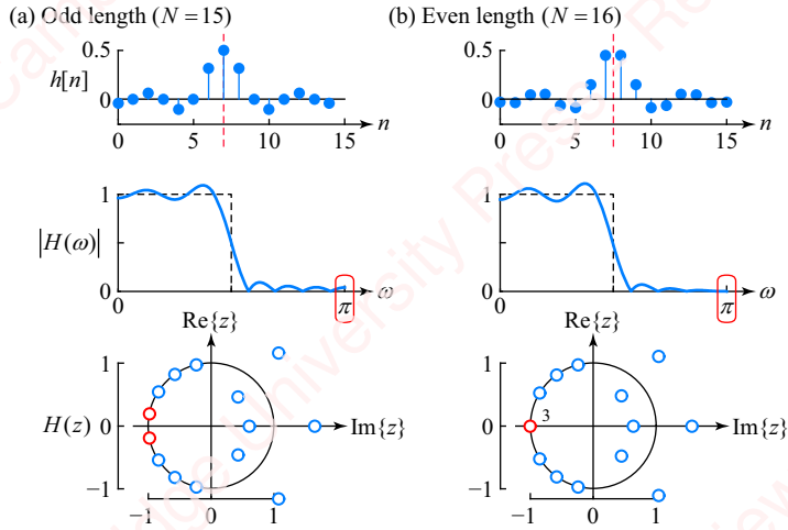
Figure 7.4 Even- and odd-length casual filters
