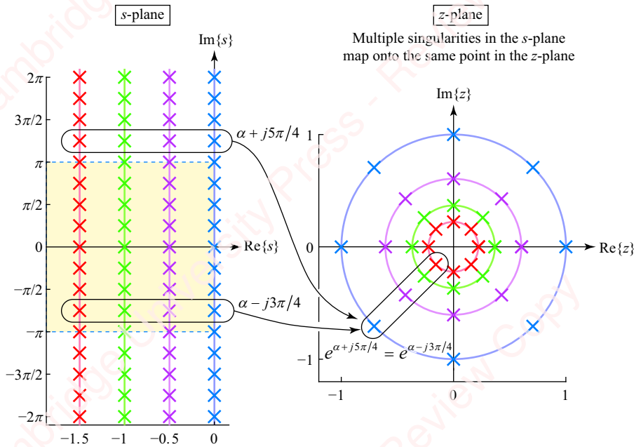
Figure 8.20 Impulse-invariance mapping the s-plane into the z-plane
